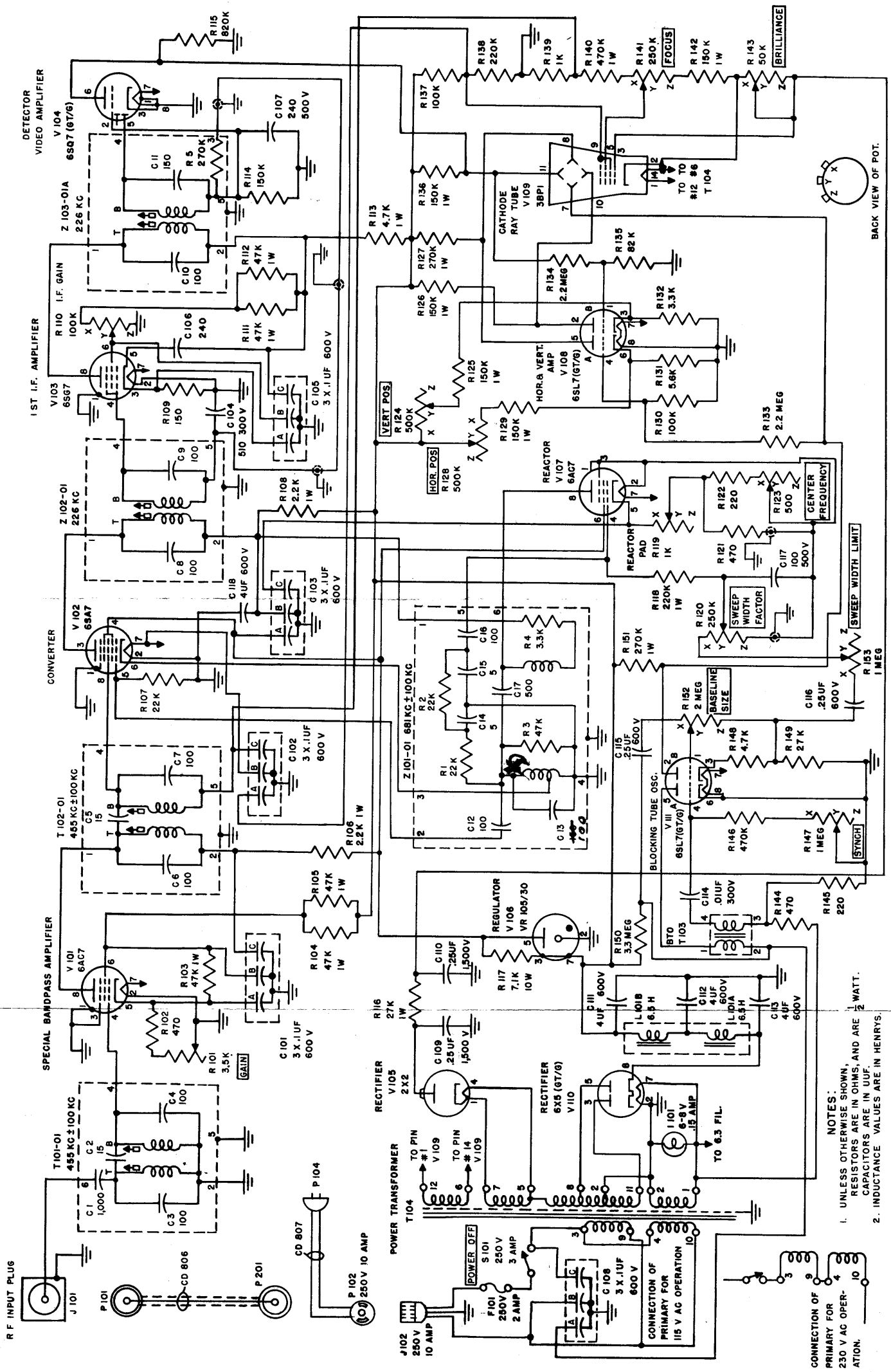
Figure 90.1 (Added) Panoramic Adaptor BC-1031-C, circuit diagram (equipment delivered on Order No. 21797-Phila-50).
